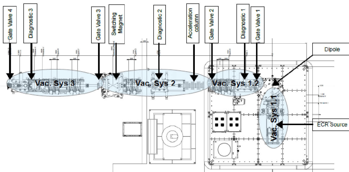
Block diagram of Vacuum system@ HFIBF
