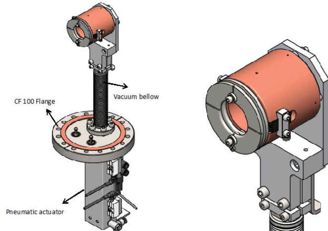
Description of Faraday cup
