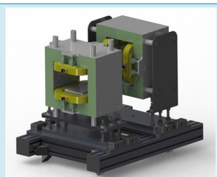
View of wobbler magnet
