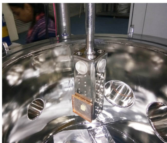
Sample ladder/holder mounted in the chamber: (a) Pre-implanted rice seeds (b) Seeds after implantation
